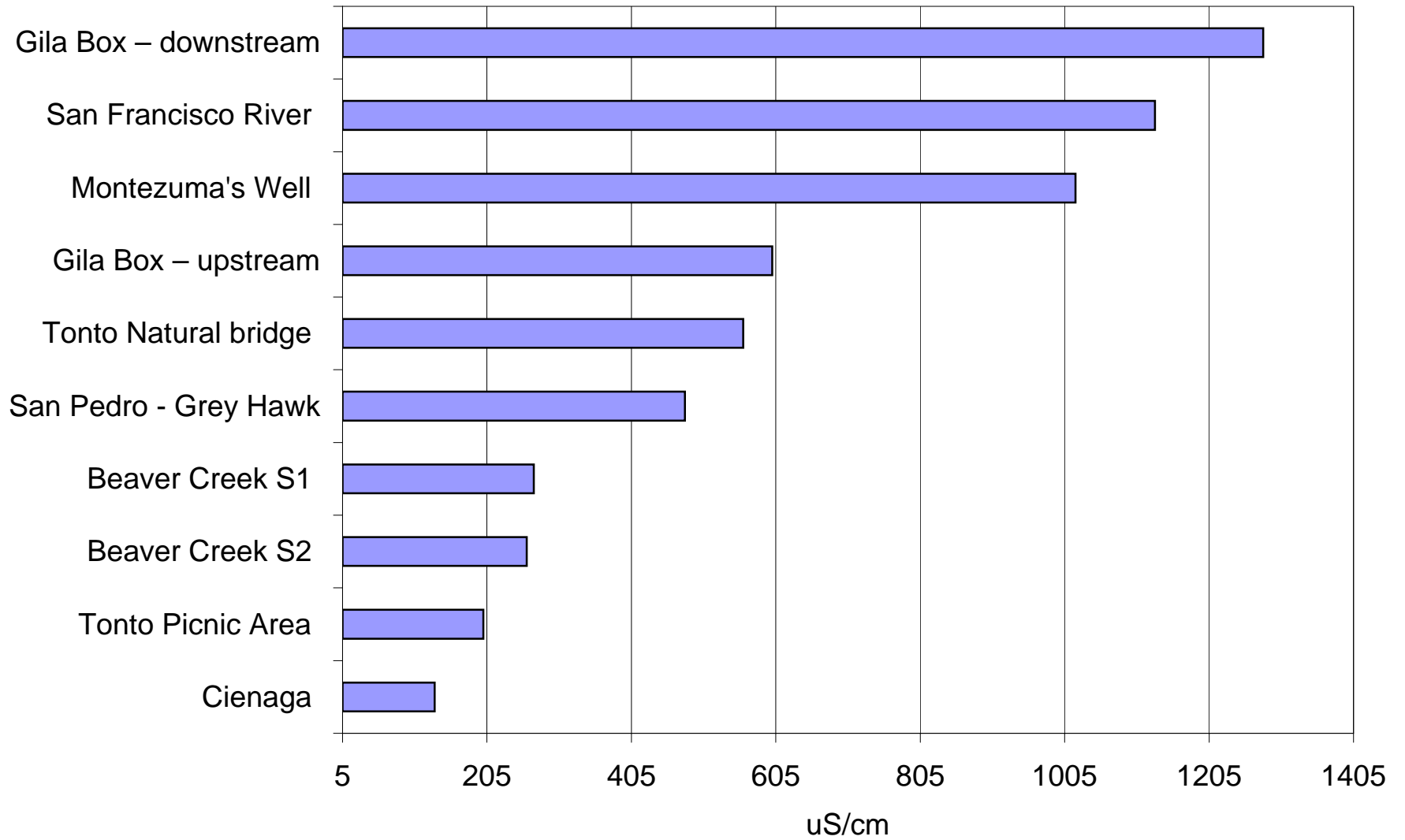
RRE 2008 - Water electrical conductivity
