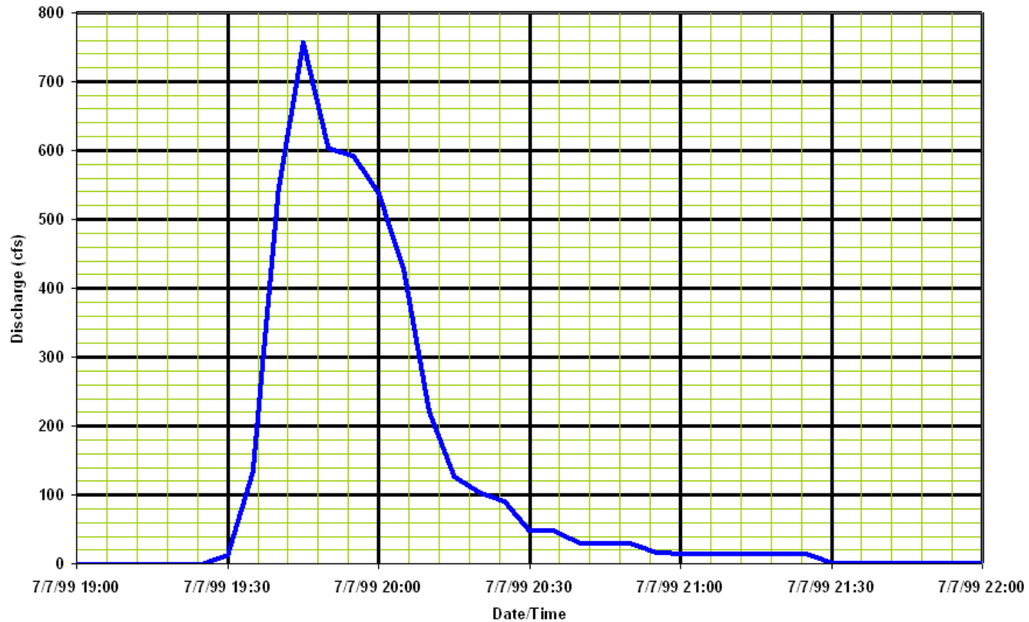
South Mountain Fan - Flood of July 7, 1999
